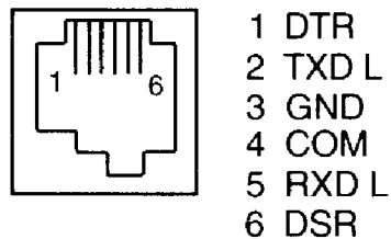
Figure B-2 Comm2 and Comm3—MMJ Ports
