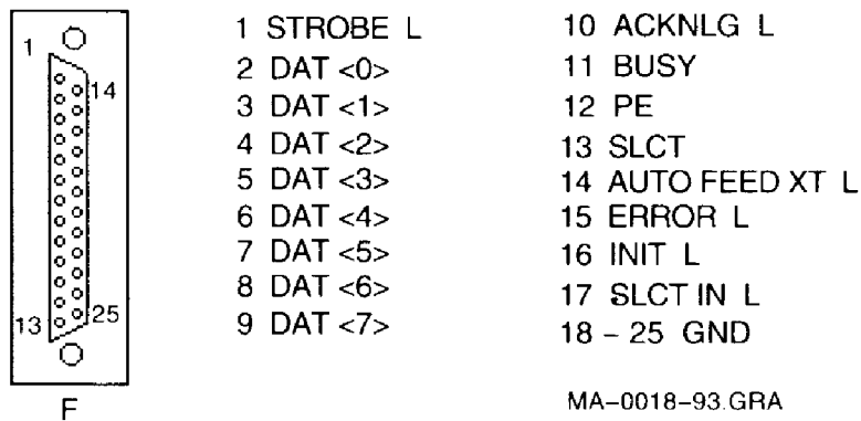
Figure B-3 Parallel Printer Port (Bidirectional)
