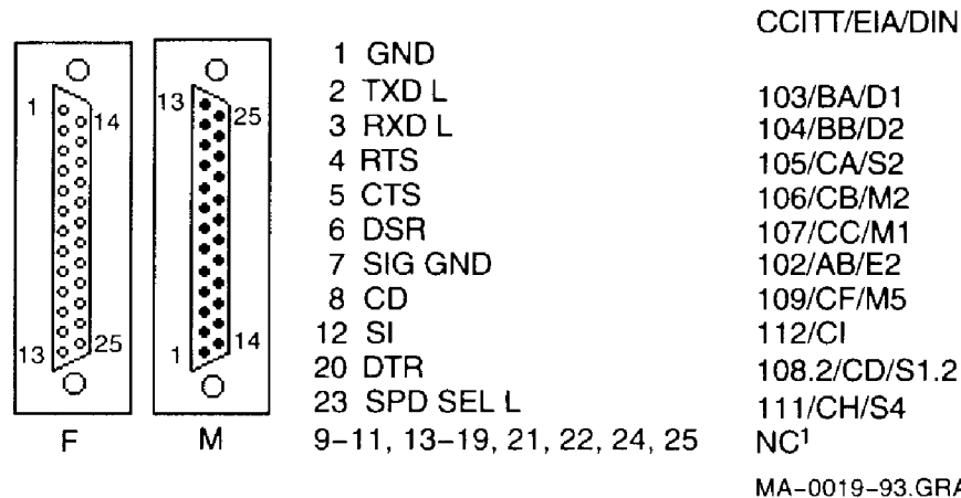
Figure B-1 Comm1—Serial Communication/Printer Ports
